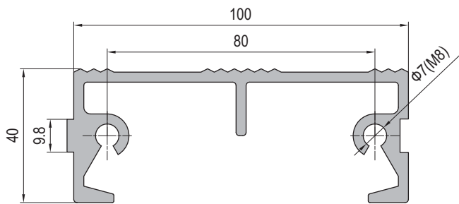
Step Profile 40x100 踏步型材 40x100
